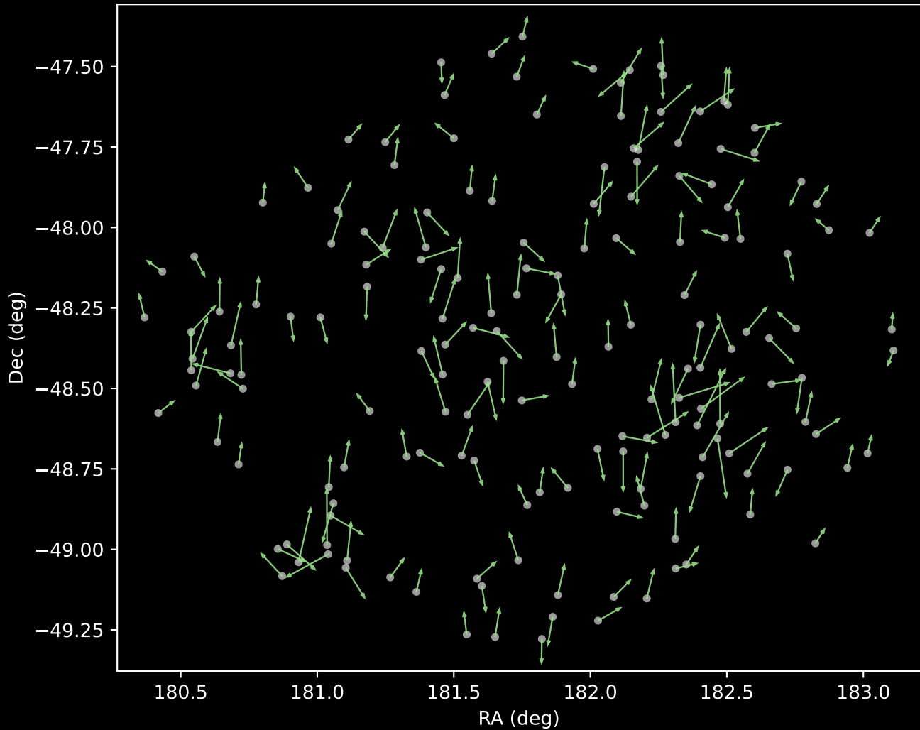
GALAH DR4 Cluster 5 Proper Motion Vectors (n=171)
