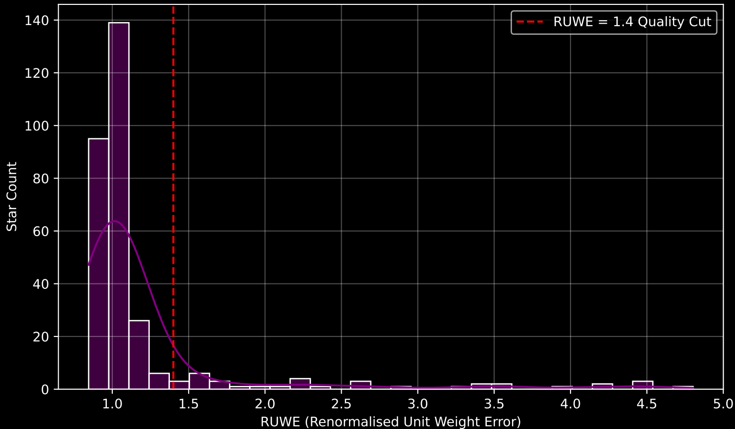
GALAH DR4 Field [626] RUWE Distribution (n= 302)
