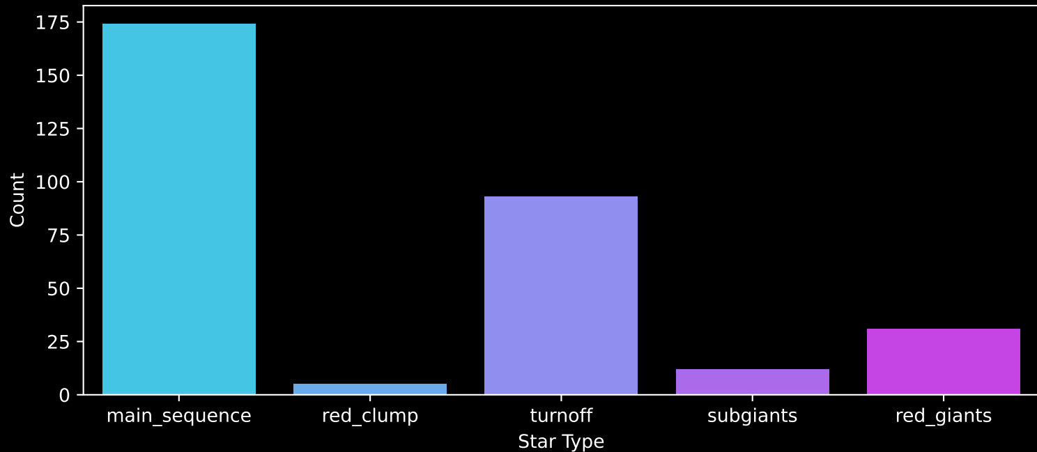
GALAH DR4 Field: [626] Count plot of Star Type
