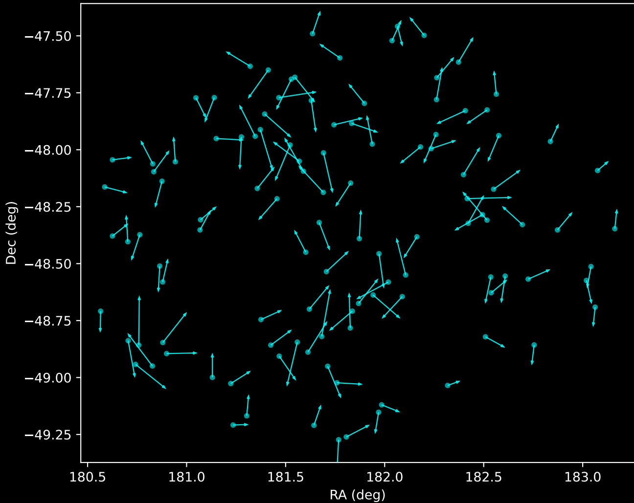
GALAH DR4 Noise Stream Proper Motion Vectors (n=112)
